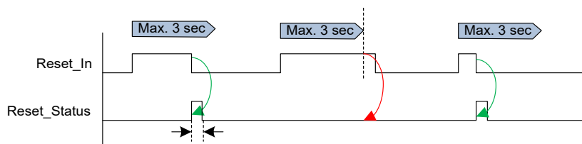
Abbildung 40: Reset-Timing
